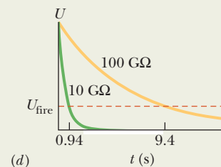
Fig. 27-17 (a) A charged car and the pavement acts like a capacitor that can discharge through the tires. (b) The effective circuit of the car-pavement capacitor, with four tire resistances R_{\text{tire}} connected in parallel. (c) The equivalent resistance R of the tires. (d) The electric potential energy U in the car-pavement capacitor decreases during discharge.
