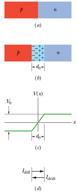
Fig. 41-12 (a) A p - n junction. (b) Motions of the majority charge carriers across the junction plane uncover a space charge associated with uncompensated donor ions (to the right of the plane) and acceptor ions (to the left). (c) Associated with the space charge is a contact potential difference V_0 across d_0 . (d) The diffusion of majority carriers (both electrons and holes) across the junction plane produces a diffusion current I_{\text{diff}} . (In a real p - n junction, the boundaries of the depletion zone would not be sharp, as shown here, and the contact potential curve (c) would be smooth, with no sharp corners.)
