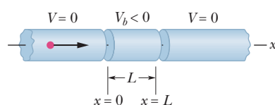
Fig. 38-14 The elements of an idealized thin wire in which an electron (the dot) approaches a negative electric potential V_b in the region x = 0 to x = L .
