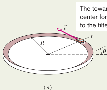
Fig. 6-11 (a) A car moves around a curved banked road at constant speed v . The bank angle is exaggerated for clarity. (b) A free-body diagram for the car, assuming that friction between tires and road is zero and that the car lacks negative lift. The radially inward component F_{Nr} of the normal force (along radial axis r ) provides the necessary centripetal force and radial acceleration.
