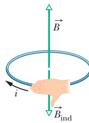
Fig. 30-5 The direction of the current i induced in a loop is such that the current's magnetic field \vec{B}_{\text{ind}} opposes the change in the magnetic field \vec{B} inducing i . The field \vec{B}_{\text{ind}} is always directed opposite an increasing field \vec{B} (a, c) and in the same direction as a decreasing field \vec{B} (b, d). The curled–straight right-hand rule gives the direction of the induced current based on the direction of the induced field.
