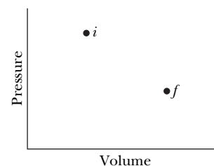
Fig. 20-2 A p - V diagram showing the initial state i and the final state f of the free expansion of Fig. 20-1. The intermediate states of the gas cannot be shown because they are not equilibrium states.
