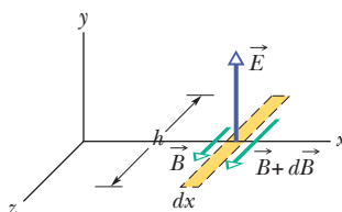
Fig. 33-7 The sinusoidal variation of the electric field through this rectangle, located (but not shown) at point P in Fig. 33-5 b , induces magnetic fields along the rectangle. The instant shown is that of Fig. 33-6: \vec{E} is decreasing in magnitude, and the magnitude of the induced magnetic field is greater on the right side of the rectangle than on the left.
