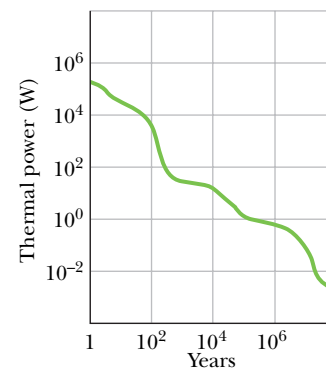
Fig. 43-7 The thermal power released by the radioactive wastes from one year's operation of a typical large nuclear power plant, shown as a function of time. The curve is the superposition of the effects of many radionuclides, with a wide variety of half-lives. Note that both scales are logarithmic.
