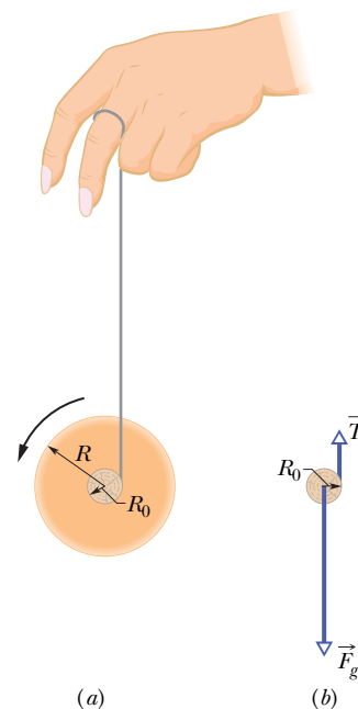
Fig. 11-9 (a) A yo-yo, shown in cross section. The string, of assumed negligible thickness, is wound around an axle of radius R_0 . (b) A free-body diagram for the falling yo-yo. Only the axle is shown.
