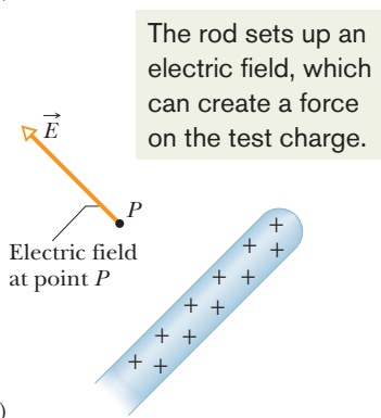
Fig. 22-1 (a) A positive test charge q_0 placed at point P near a charged object. An electrostatic force \vec{F} acts on the test charge. (b) The electric field \vec{E} at point P produced by the charged object.
