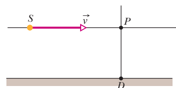
Fig. 37-12 A light source S travels with velocity \vec{v} past a detector at D . The special theory of relativity predicts a transverse Doppler effect as the source passes through point P , where the direction of travel is perpendicular to the line extending through D . Classical theory predicts no such effect.
