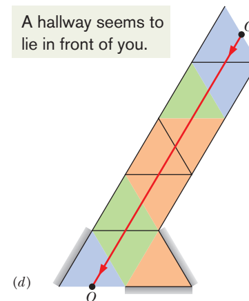
Fig. 34-7 (a) Overhead view of a mirror maze. A ray from mirror B reaches you at O by reflecting from mirror A . (b) Mirror B appears to be behind A . (c) The ray reaching you comes from you. (d) You see a virtual image of yourself at the end of an apparent hallway.
