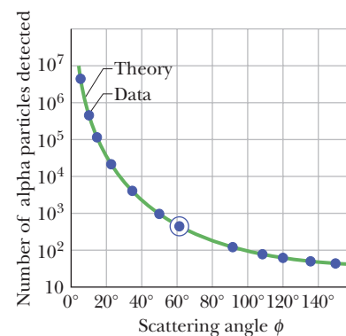
Fig. 42-2 The dots are alpha-particle scattering data for a gold foil, obtained by Geiger and Marsden using the apparatus of Fig. 42-1. The solid curve is the theoretical prediction, based on the assumption that the atom has a small, massive, positively charged nucleus. The data have been adjusted to fit the theoretical curve at the experimental point that is enclosed in a circle.
