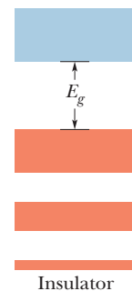
Fig. 41-4 The band–gap pattern for an insulator; filled levels are shown in red and empty levels in blue.
