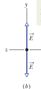
Fig. 33-9 (a) The plane of oscillation of a polarized electromagnetic wave. (b) To represent the polarization, we view the plane of oscillation head-on and indicate the directions of the oscillating electric field with a double arrow.
