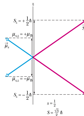
Fig. 40-6 The allowed values of S_z and \mu_z for an electron.
