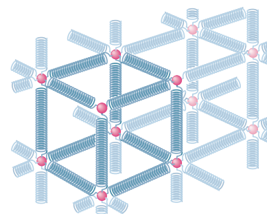
Fig. 12-9 The atoms of a metallic solid are distributed on a repetitive three-dimensional lattice. The springs represent interatomic forces.
