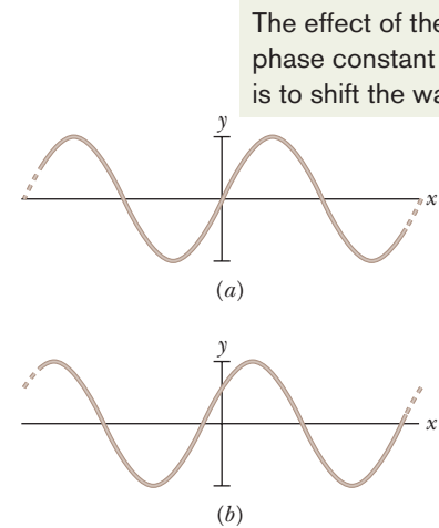
Fig. 16-6 A sinusoidal traveling wave at t = 0 with a phase constant \phi of (a) 0 and (b) \pi/5 rad.
