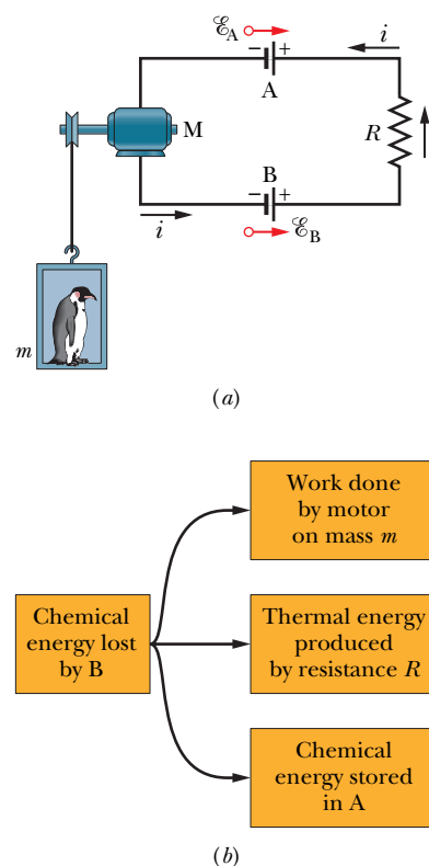
Fig. 27-2 (a) In the circuit, \mathcal{E}_B > \mathcal{E}_A ; so battery B determines the direction of the current. (b) The energy transfers in the circuit.
