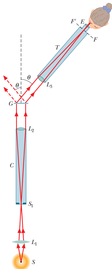
Fig. 36-23 A simple type of grating spectroscopy used to analyze the wavelengths of light emitted by source S .
