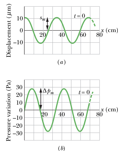
Fig. 17-6 (a) A plot of the displacement function (Eq. 17-12) for t = 0 . (b) A similar plot of the pressure-variation function (Eq. 17-13). Both plots are for a 1000 Hz sound wave whose pressure amplitude is at the threshold of pain.
