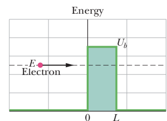
Fig. 38-15 An energy diagram containing two plots for the situation of Fig. 38-13: (1) The electron's mechanical energy E is plotted when the electron is at any coordinate x < 0 . (2) The electron's electric potential energy U is plotted as a function of the electron's position x , assuming that the electron can reach any value of x . The nonzero part of the plot (the potential barrier) has height U_b and thickness L .
