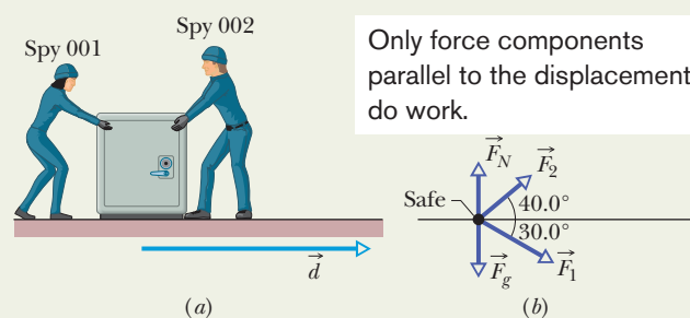
Fig. 7-4 (a) Two spies move a floor safe through a displacement \vec{d} . (b) A free-body diagram for the safe.
