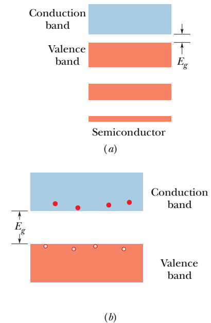
Fig. 41-9 (a) The band-gap pattern for a semiconductor. It resembles that of an insulator (see Fig. 41-4) except that here the energy gap E_g is much smaller; thus electrons, because of their thermal agitation, have some reasonable probability of being able to jump the gap. (b) Thermal agitation has caused a few electrons to jump the gap from the valence band to the conduction band, leaving an equal number of holes in the valence band.
