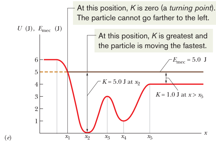
Fig. 8-9 (a) A plot of U(x) , the potential energy function of a system containing a particle confined to move along an x axis. There is no friction, so mechanical energy is conserved. (b) A plot of the force F(x) acting on the particle, derived from the potential energy plot by taking its slope at various points. (c)–(e) How to determine the kinetic energy. (f) The U(x) plot of (a) with three possible values of E_{\text{mec}} shown.
