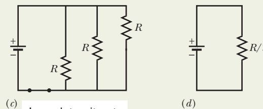
Fig. 30-18 (a) A multiloop RL circuit with an open switch. (b) The equivalent circuit just after the switch has been closed. (c) The equivalent circuit a long time later. (d) The single-loop circuit that is equivalent to circuit (c).
